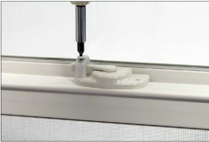
Figure 3: Install the lock limiter and tighten the screw (#6 x 1 1/4" Torx head).
