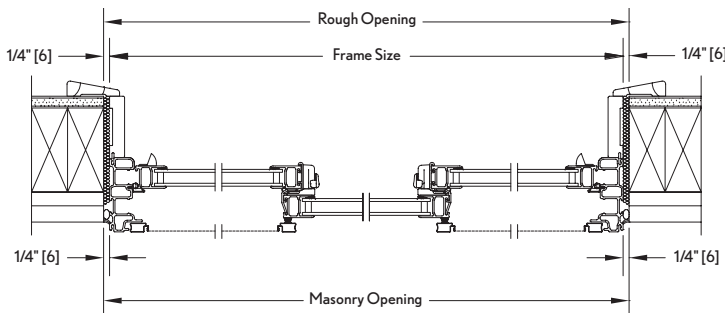
Triple Sash XOX Operator Jamb
