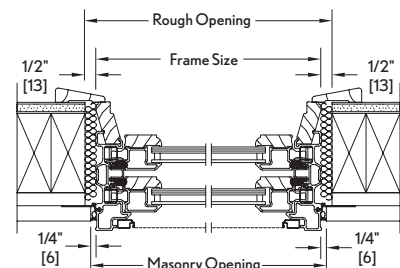
Operator Jamb
