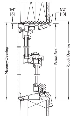
Operator Head Jamb and Sill
