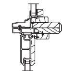
Direct Glaze Polygon/Transom Over Outswing French Door
