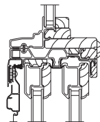
Direct Glaze Transom Over Sliding Patio Door
